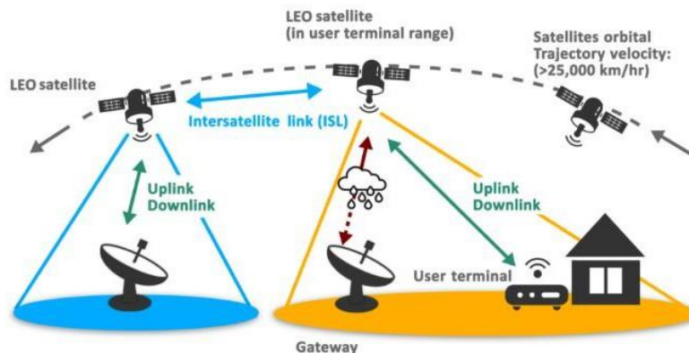
Figure 1: LEO System Architecture [13]
