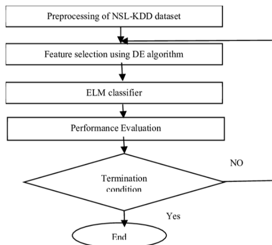
Figure 4: Processing of NSL-KDD (2021)
