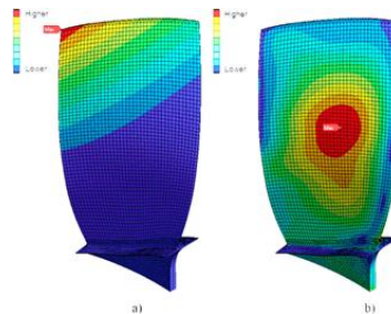
Figure 2: Damage Prediction on Turbofan Blade as Static Plate
