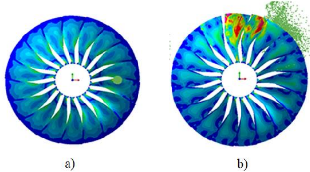
Figure 4: Damage Prediction on Turbofan Blade as Rotating Plate
