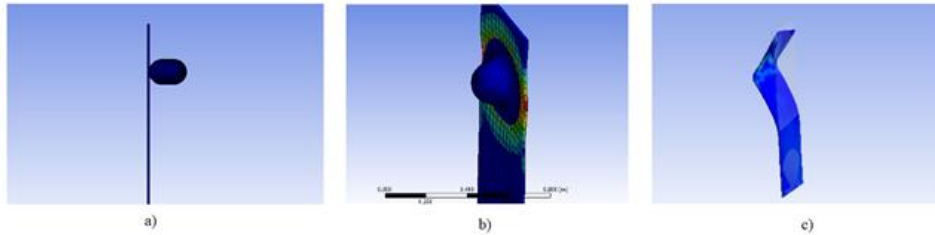
Figure 2: Damage Prediction on Turbofan Blade as Flat Plate
