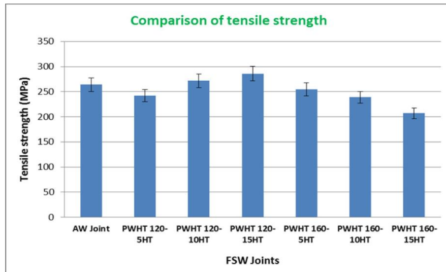
Figure2: Comparison Of Tensile Strength
