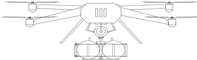
Figure4: Fire Fighting Drone Model with Ball Extinguisher
